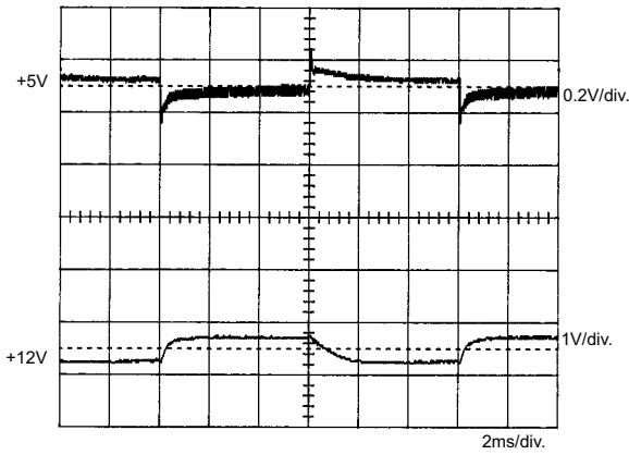
+5V steps from 1A to 5A other output at 60% load
