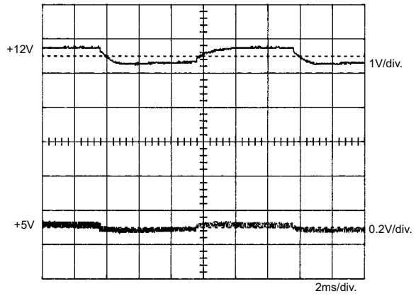
+12V steps from 0.46A to 2.3A other output at 60% load
