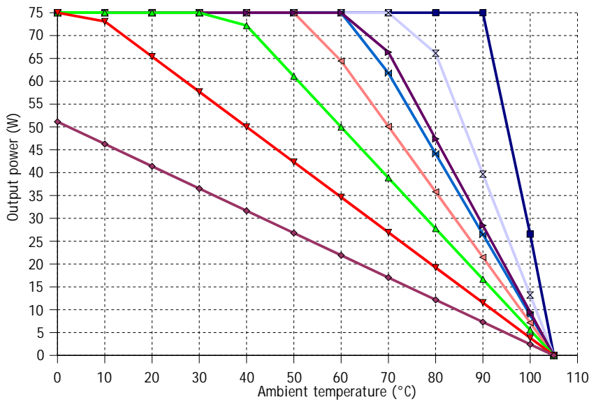
MGDS-75-H-x Series Thermal Curves
