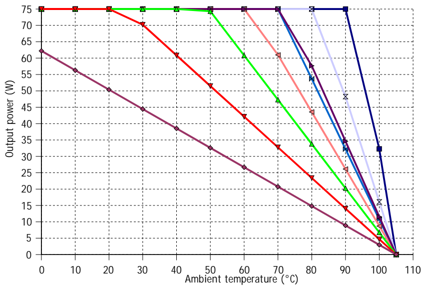
MGDS-75-O-x Series Thermal Curves
