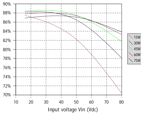
Typical efficiency MGDS750F at 25°C
